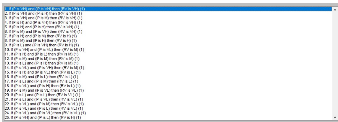
Figure 5. Rule block and rules.
